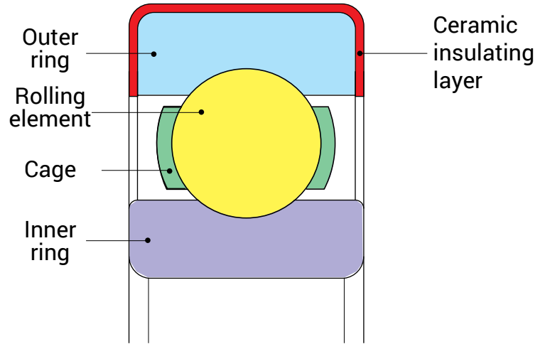
Deep Groove Ball Bearing
