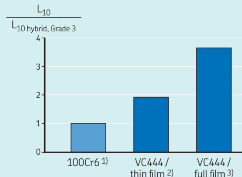
Fatigue life tests under thin-film and full-film lubrication conditions
