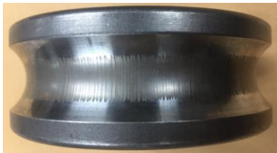
Picture 1: Electrical Discharge Damage (Fluting)
